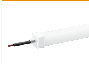
AC167-EC5-F Silicone end cap front entry with 30cm (0.98ft) cable, 2 pin
