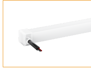
AC167-EC5-S Silicone end cap side entry with 30cm (0.98ft) cable, 2 pin
